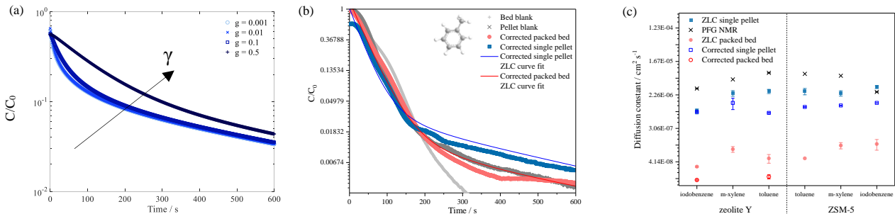
Fig. 1. (a) Simulated diffusion curves with increasing fluid-phase hold-up, \gamma (b) Diffusion models fitted to experimental toluene data from zeolite Y (c) A comparison of NMR and ZLC diffusion constants.
